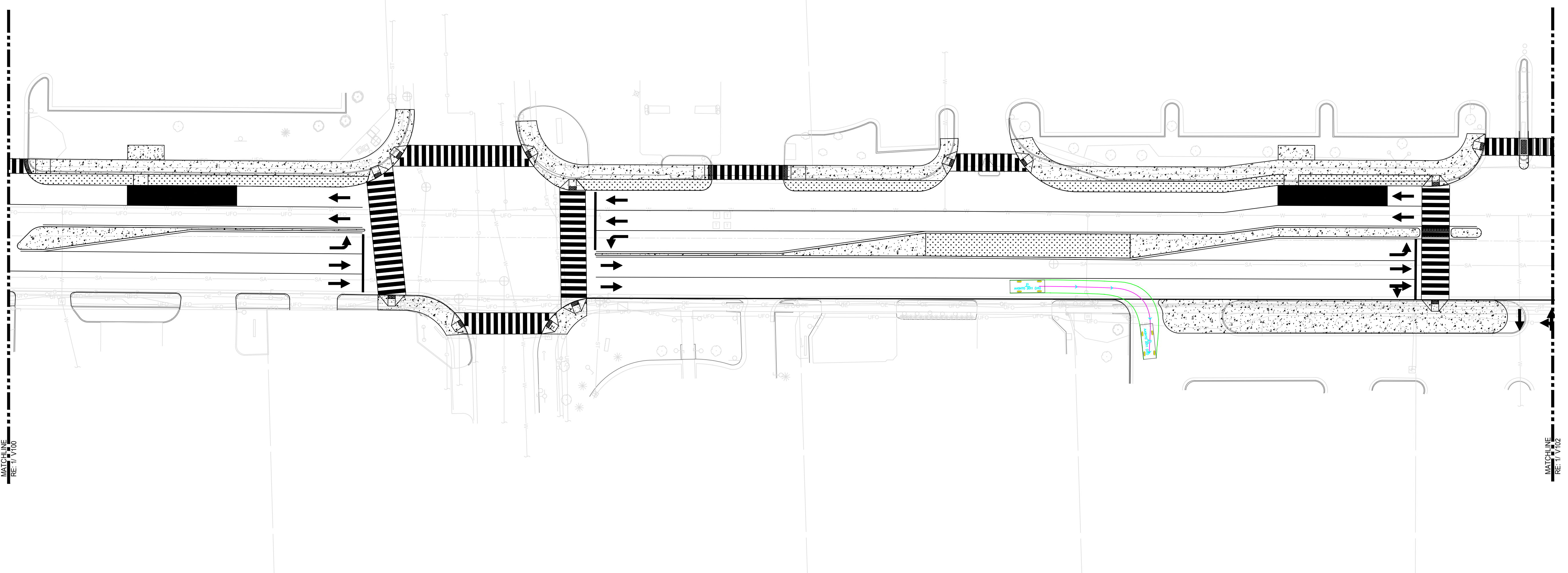
1 ELDEN STREET - PLAN SCALE: 1" = 30'
